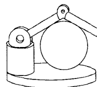
Figure 2: Robust hold of an object by means of an enveloping, "whole-arm" grasp.
