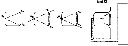
Figure 4: Example of asymptotic reproducible contact forces ( \mathcal{F}_{hr} \subseteq \ker(\mathbf{G}) ).
