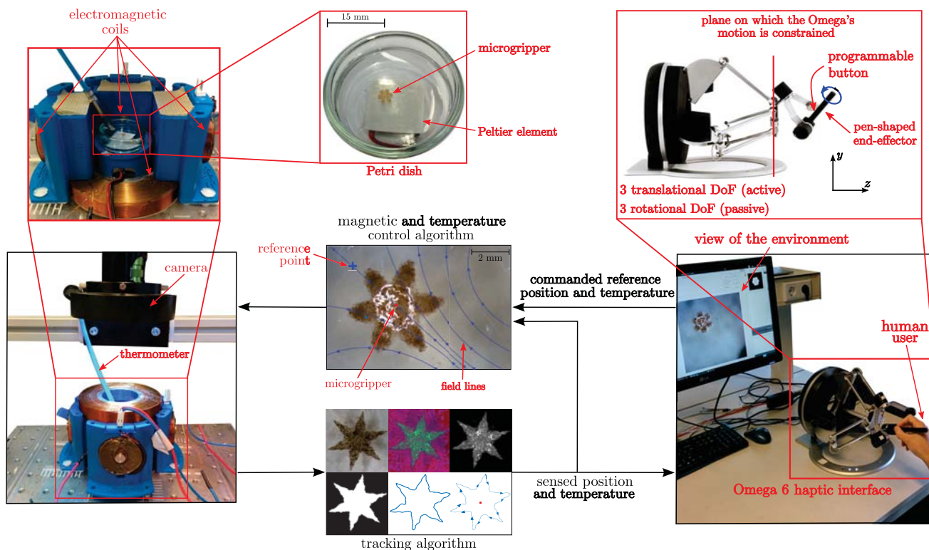
Fig. 2. Teleoperation of magnetic soft grippers with haptic feedback. The image-guided algorithm tracks the position of the gripper in the remote environment using a high-resolution camera and a Fourier-descriptors-based algorithm. A 6-DoF grounded haptic interface then provides the human operator with haptic feedback about the interaction of the gripper with the remote environment. At the same time, it enables the operator to intuitively control the reference position and grasping configuration of the gripper. Finally, magnetic and thermal control algorithms regulate the position and grasping configuration of the gripper.
