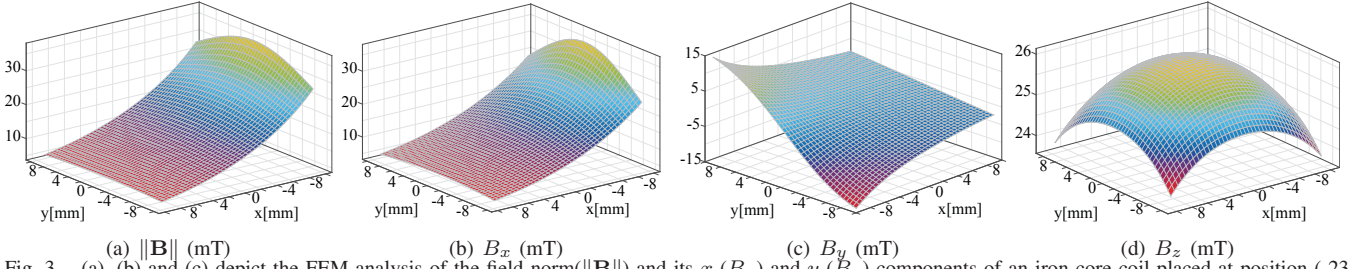
Fig. 3. (a), (b) and (c) depict the FEM analysis of the field norm( \|\mathbf{B}\| ) and its x ( B_x ) and y ( B_y ) components of an iron-core coil placed at position (-23 mm; 0 mm) with respect to the graph. The coil is controlled with a current of 1 A. (d) shows the z ( B_z ) component of the field when controlling the air-core upper coil with a current of 1 A. Given the symmetry of the setup (Fig. 2), the field generated by the other coils can be obtained by properly rotating the ones shown here.
